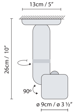
CAPSULE SURFACE QR-CB 51 CAPSULE SURFACE (GZ10)
