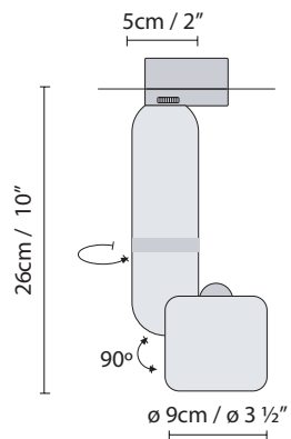
CAPSULE TRACK QR-CB 51 CAPSULE TRACK (GZ10)
