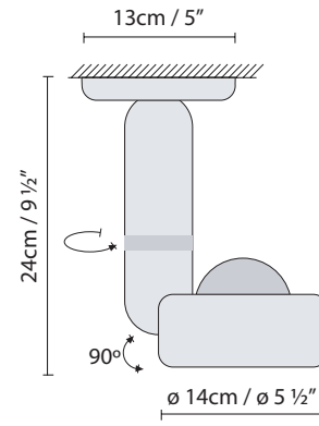
CAPSULE SURFACE QR-111
