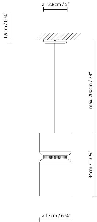
ASPEN S17A LED / ASPEN S17A (E27)
