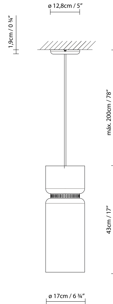
ASPEN S17B LED / ASPEN S17B (E27)
