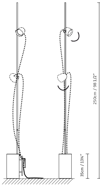
Sample 1: Speers Outdoor F Accesory + 2 Light Source
