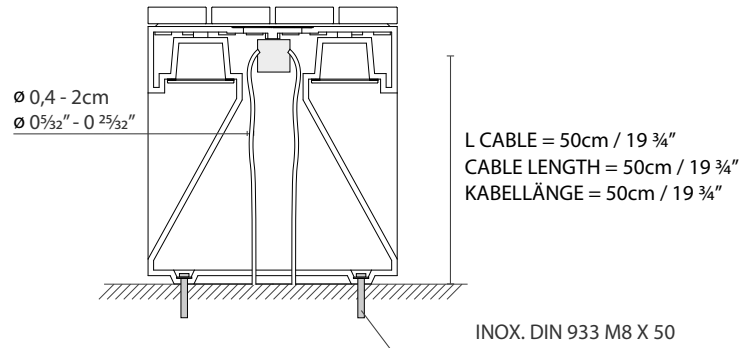
LAP BENCH 45A LED / LAP BENCH 45B LED LAP BENCH 45A FLUO / LAP BENCH 45B FLUO
