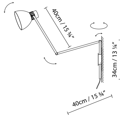
W40 PLUG-IN
