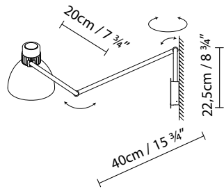
W20 PLUG-IN
