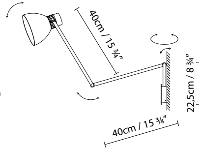
W40 PLUG-IN
